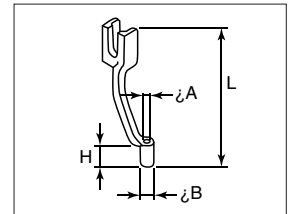
Intermediate presser
